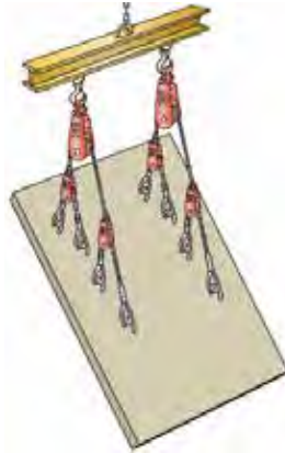
Lifting and rotating tilt panels
