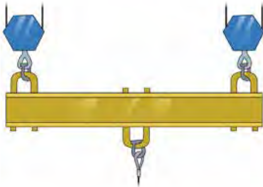
Lifts using load equalising gear
